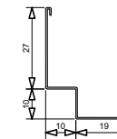
WASL Wall Angle
