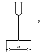
DX2-600 Cross Tee
