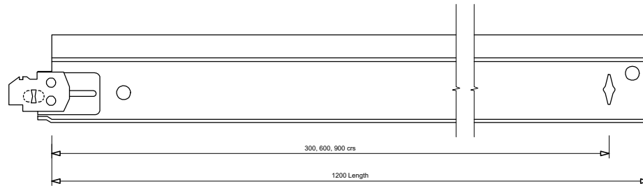
DX2/3 Cross Tee
